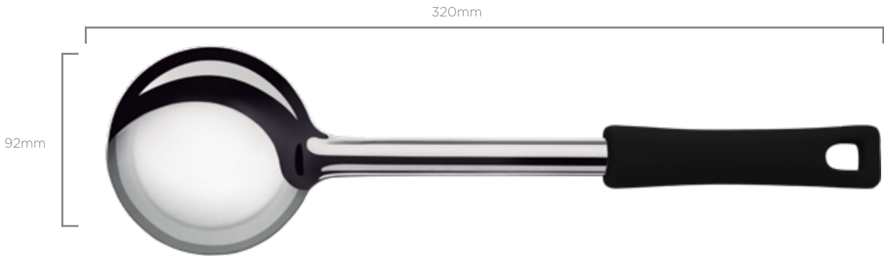
Concha terrina 85ml Soup ladle / Cucharón terrina Ref: 18.0710.EE.CC
